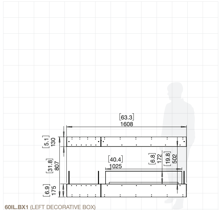
60IL.BX1 (LEFT DECORATIVE BOX)
